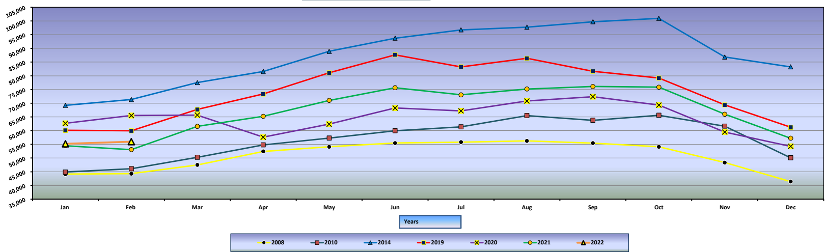
Average Daily Truck Traffic All ATR's
