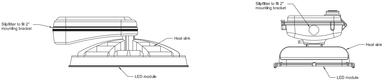
Typical LED Luminaire Details
