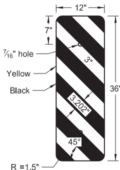
Object Marker Left OM-3L (C) Type III
