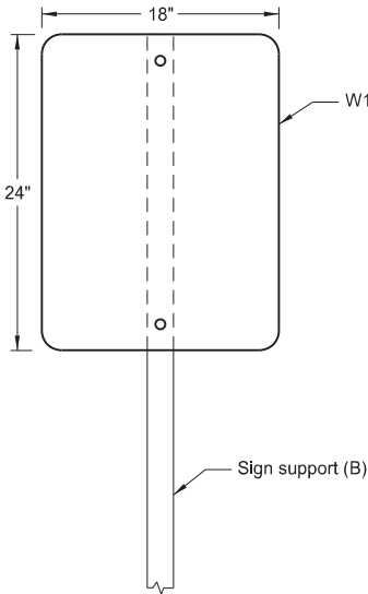
Chevron Single Sign Assembly (B) Use 2x2x12ga. perforated tube single sign support and 2.25x2.25x12ga. perforated tube anchor unit.
