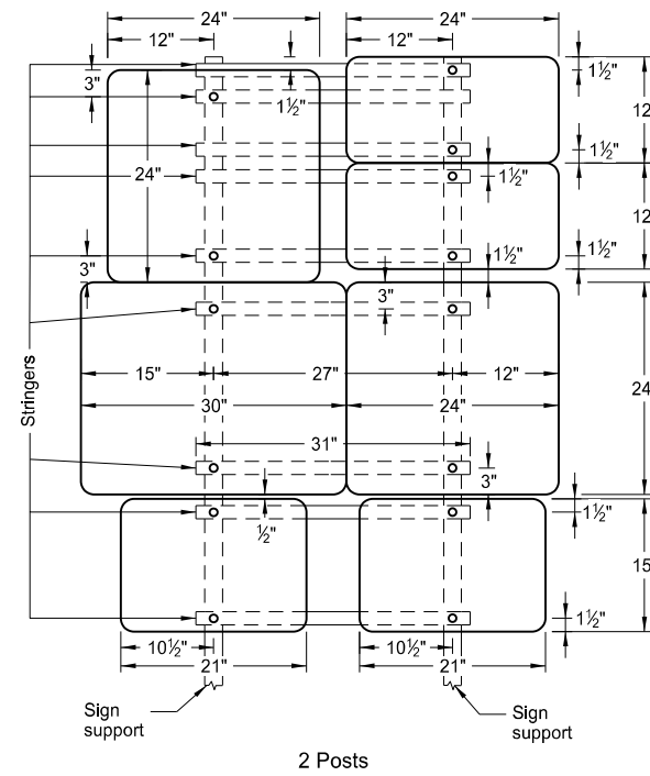
ASSEMBLY NO. 433
