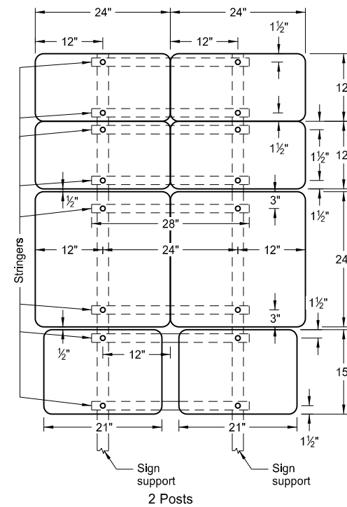
ASSEMBLY NO. 429
