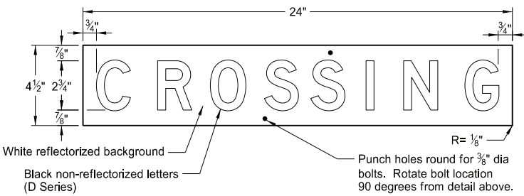
Railroad Crossing Sign Details
