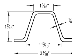
Steel Post Detail (approx. 2 lb/ft)
