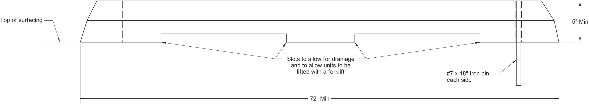
SIDE VIEW
