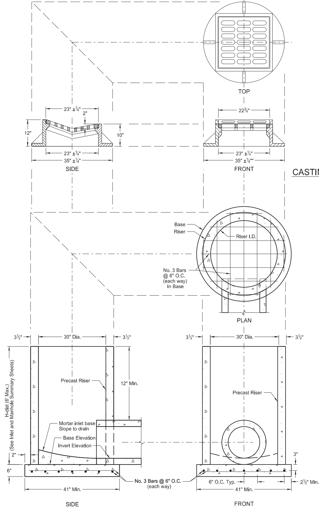
BASE & RISER DETAILS
