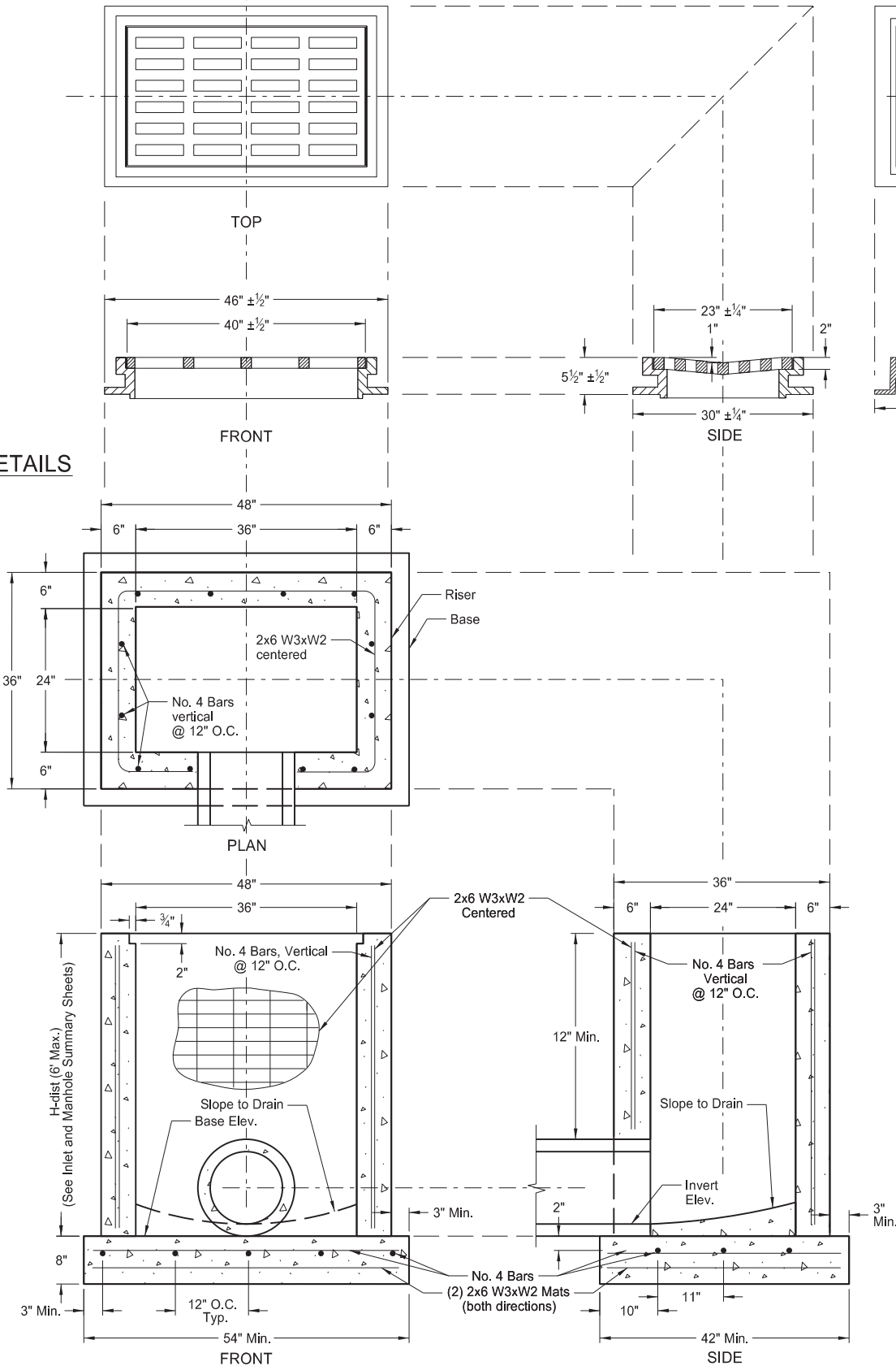
BASE & RISER DETAILS
