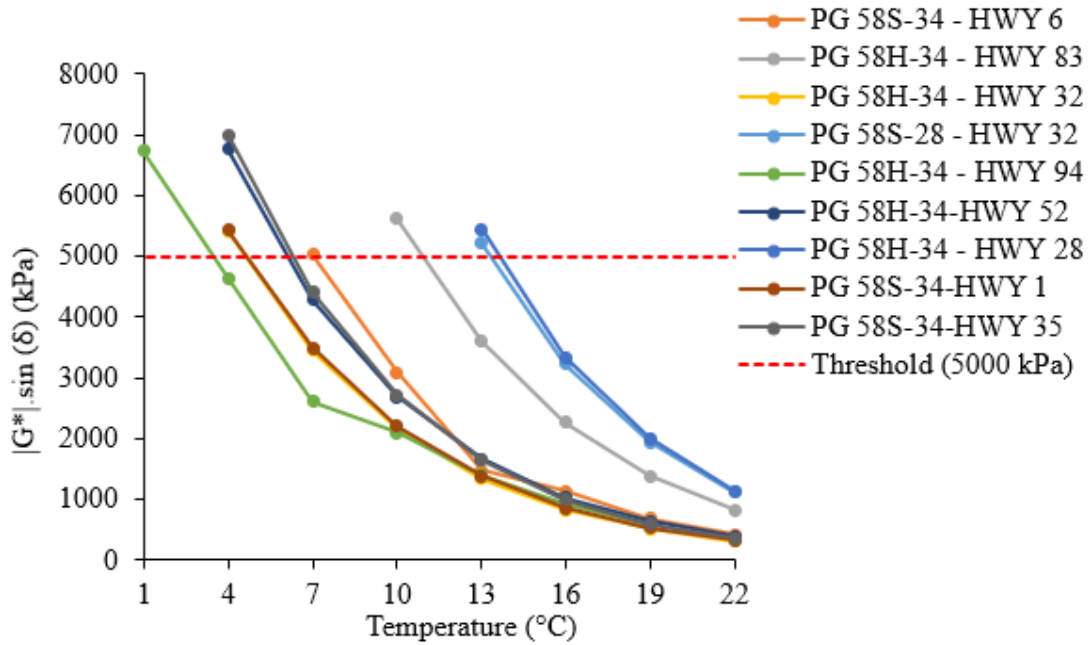
Figure 4.10: |G^*| \cdot \sin(\delta) values of the PAV-Aged Binder
