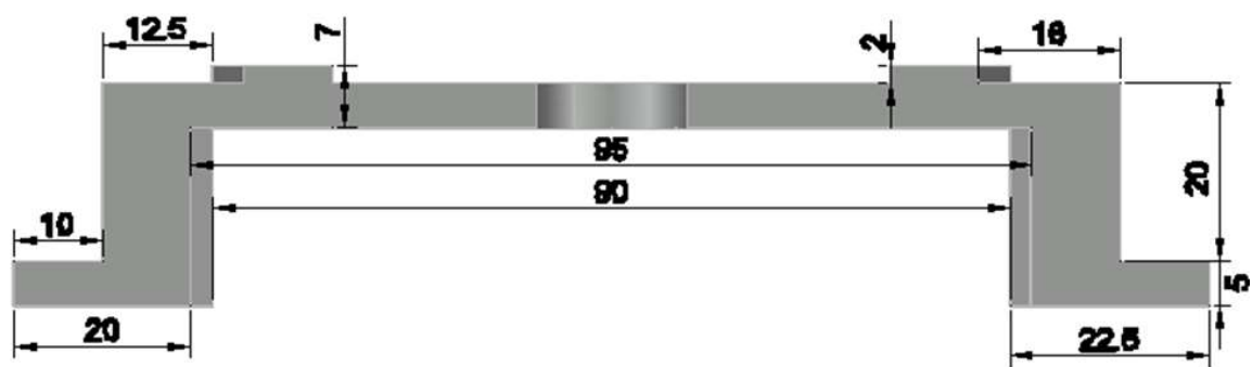
Front View
