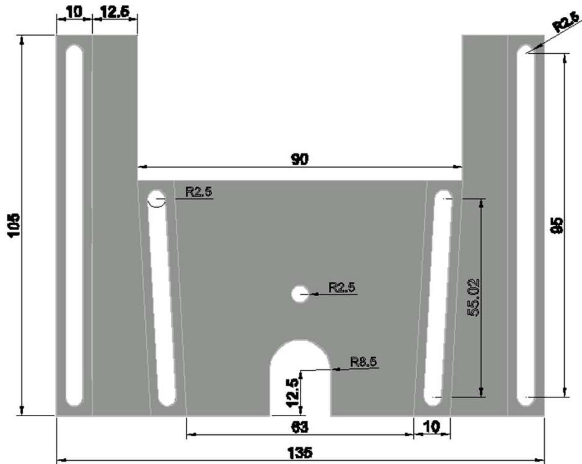
Top-Down View
