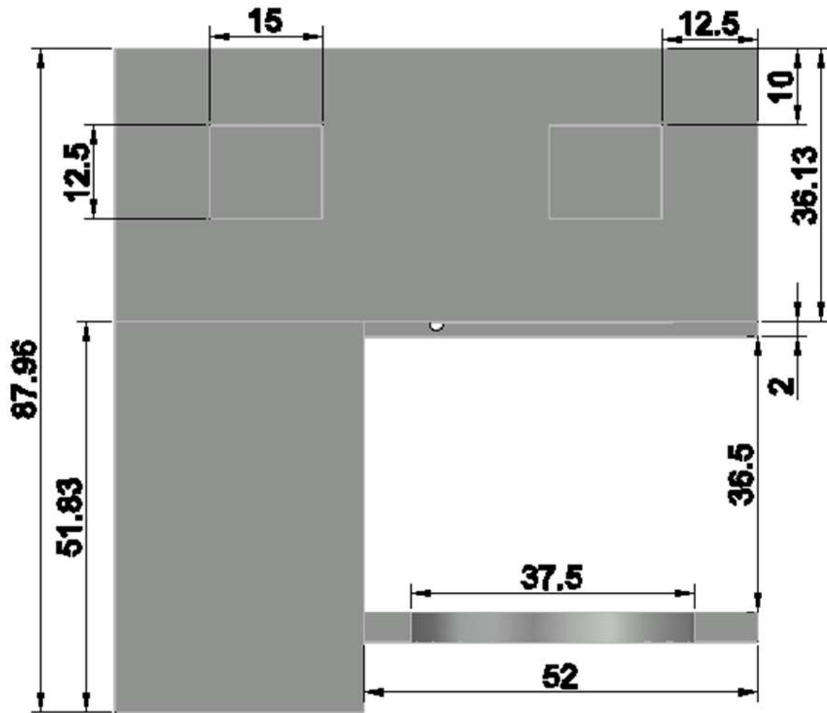
Top-Down View
