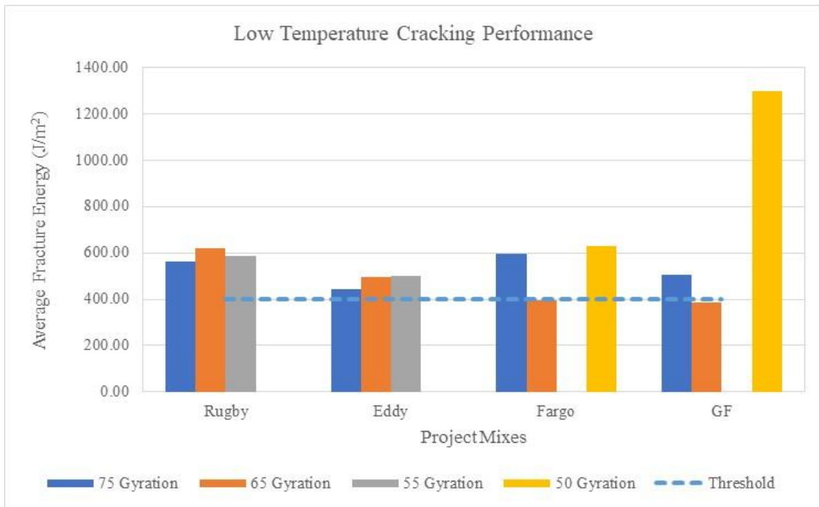
Figure 37. Overall Low Temperature Cracking Performance Results
