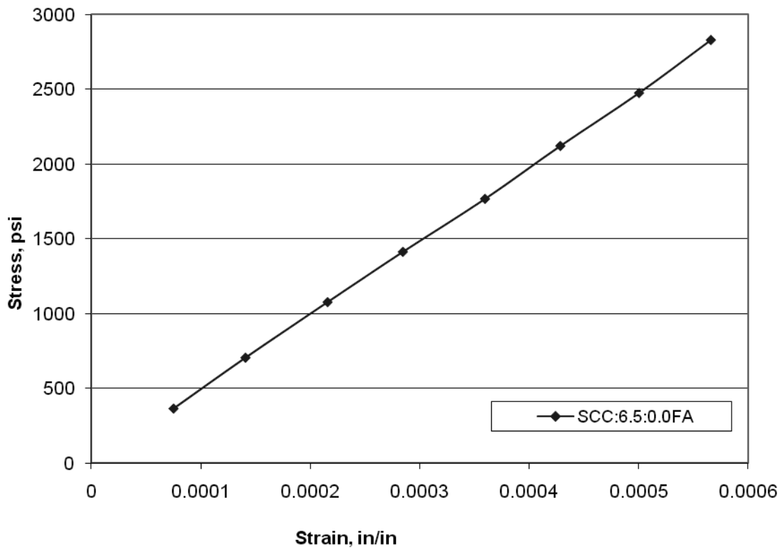
Figure AV.6: Stress vs. strain relationship
