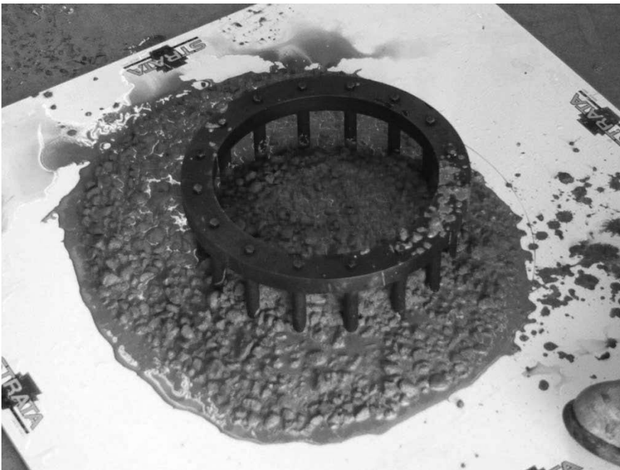
Figure 21: Slump flow with J-Ring VBI = 3.
