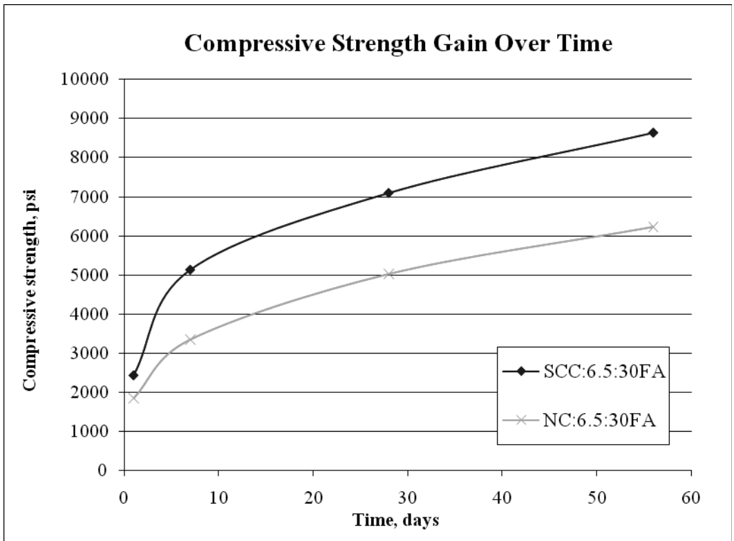
Figure 29: Compressive Strength of SCC:6.5:30FA vs. NC:6.5:30FA
