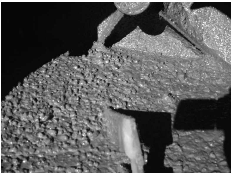
Figure 16: Very viscous SCC mix
