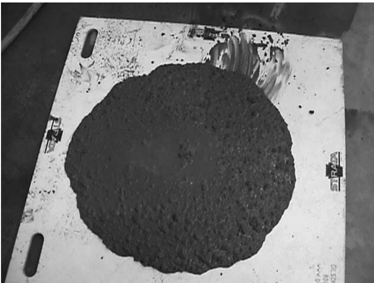
Figure 14: SCC mix with VSI=0.5, evidence of bleeding in the center
