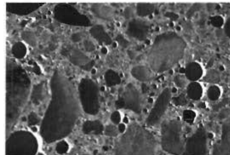
Magnification: 30x Description: Overall hardened air content, 5.4% total
