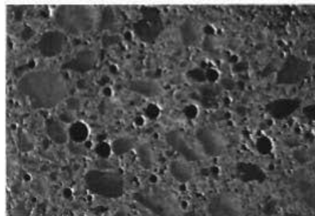
Magnification: 30x Description: Overall hardened air content, 3.5% total
