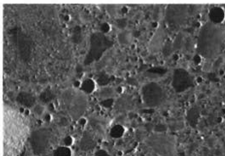
Magnification: 30x Description: Overall hardened air content, 4.6% total
