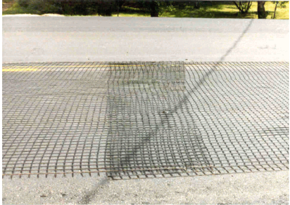
Photo 3. View of the geogrid overlap.
