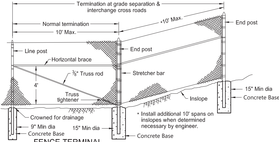
FENCE TERMINAL
