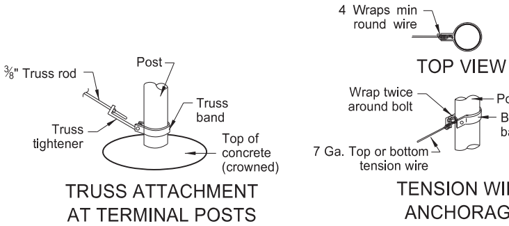
BRACE & TRUSS ATTACHMENT
