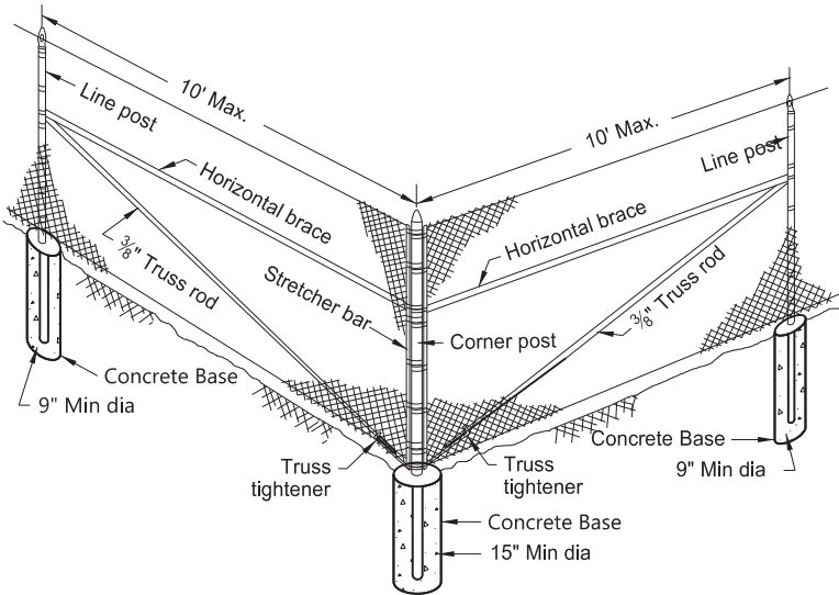
CORNER ASSEMBLY
