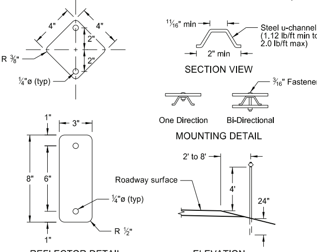
REFLECTOR DETAIL
