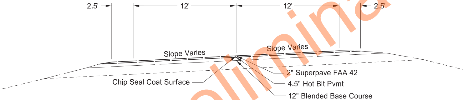
Existing Typical Section - Curve
