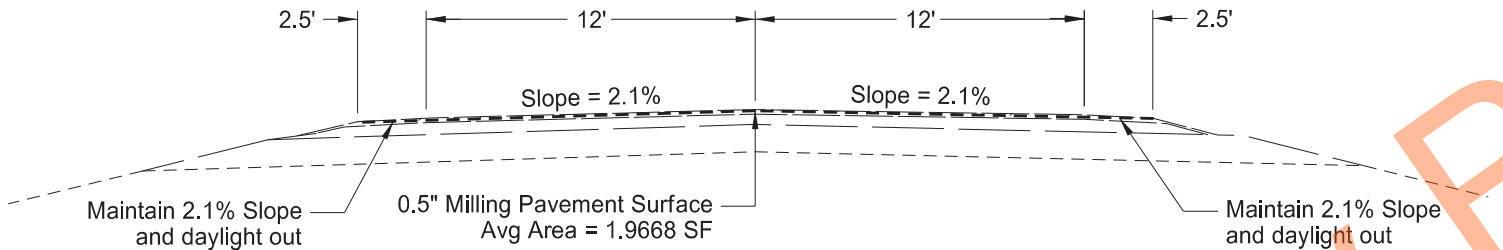
Milling Typical Section - Tangent
