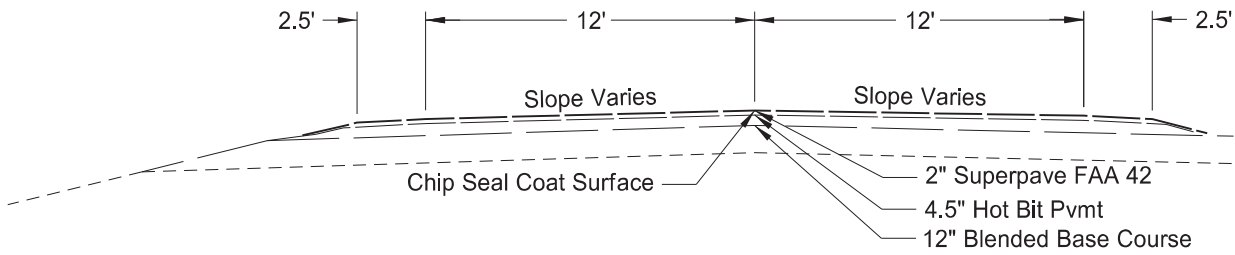
Existing Typical Section - Tangent
