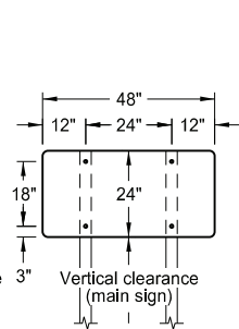
48" x 24" SIGN
