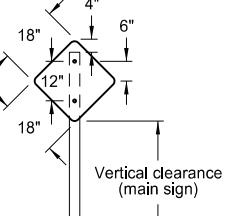
18" x 18" DIAMOND SIGN
