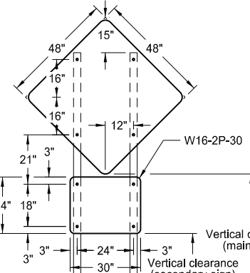
48" x 48" DIAMOND SIGN (with 30" x 24" secondary sign)
