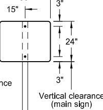
30" x 24" SIGN
