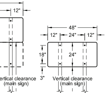
60" x 24" SIGN
