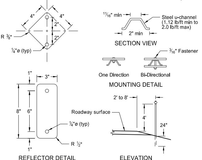
REFLECTOR DETAIL
