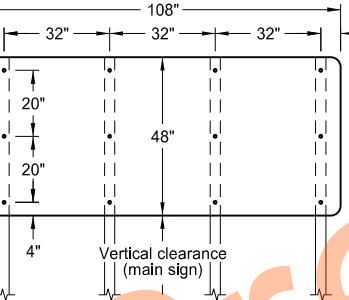
108" x 48" SIGN
