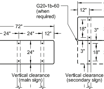
72" x 24" SIGN
