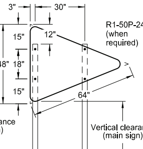
W14-3-64 - PENNANT SIGN
