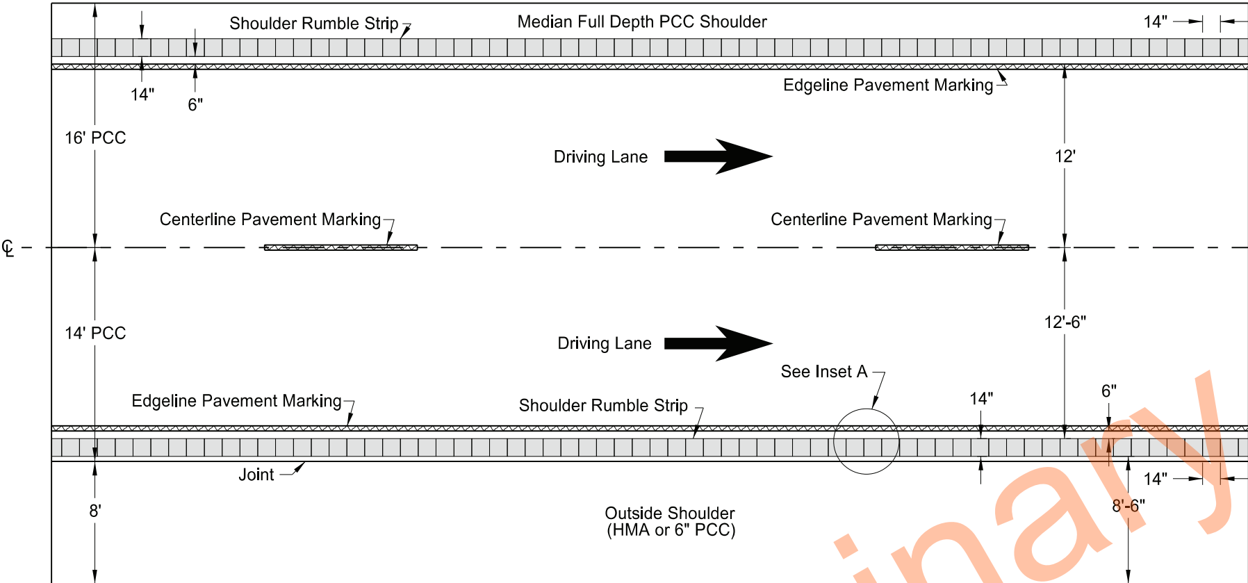
30' Wide Full Depth PCC with 8' Wide HMA Outside Shoulder
