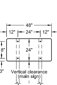
48" x 24" SIGN
