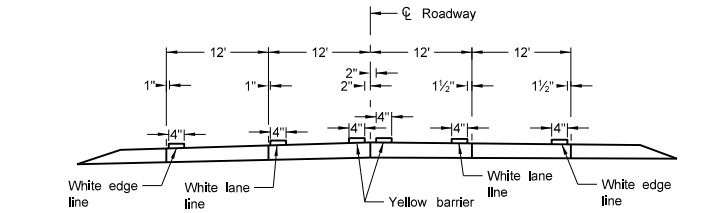
URBAN FIVE LANE SECTION Asphalt Section
