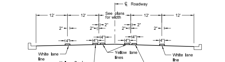
RURAL FIVE LANE ROADWAY Asphalt Section
