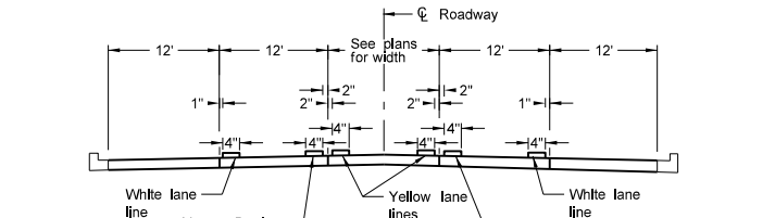
RURAL FIVE LANE ROADWAY Concrete Section
