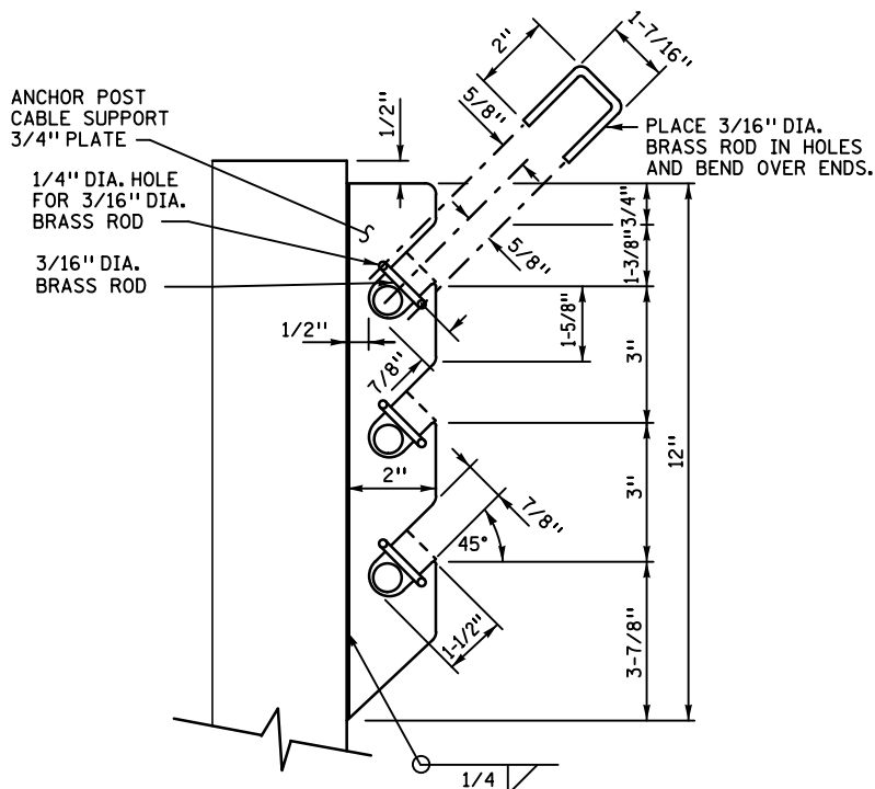
SIDE VIEW OF POST TOP
