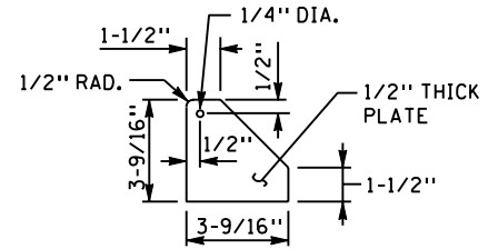
EXTERNAL STIFFENER PLATE
