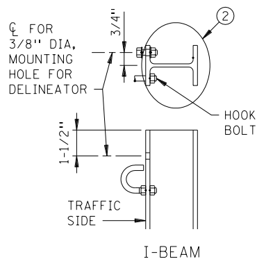
LINE POST DELINEATOR DETAILS
