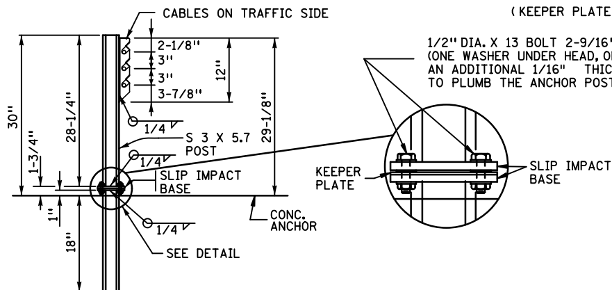
SIDE VIEW ANCHOR POST DETAIL (SHOWN FOR LEFT HANDED ANCHOR)
