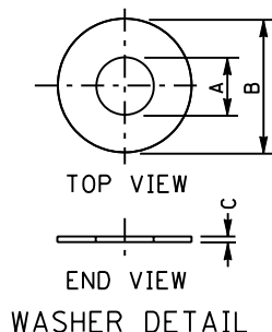
WASHER DETAIL
