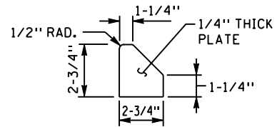
INTERNAL STIFFENER PLATE
