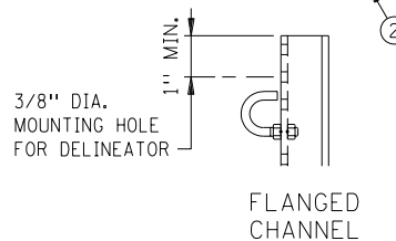
LINE POST DELINEATOR DETAILS
