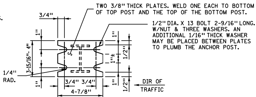
SLIP IMPACT BASE (KEEPER PLATE NOT SHOWN)
