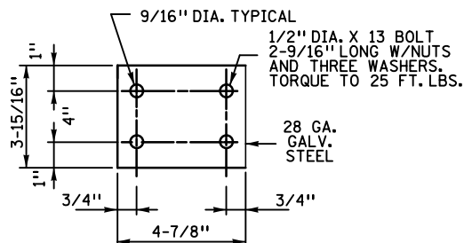
KEEPER PLATE (INSERT BETWEEN TOP AND BOTTOM PLATES OF SLIP IMPACT BASE)
