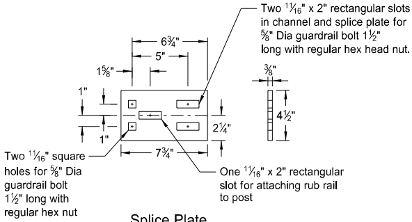
Splice Plate
