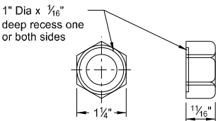
5/8" Dia recess nut
