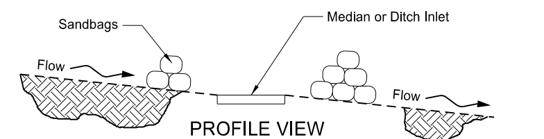
SANDBAG PROTECTION (ON SLOPE)
