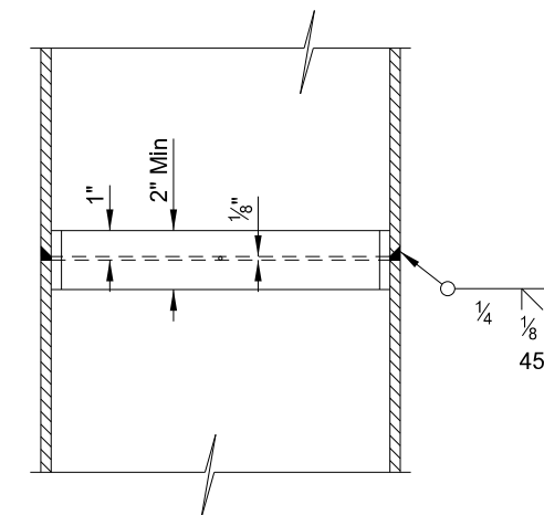
C-C STEEL-ENCASED CONCRETE PILE SPLICE DETAIL
