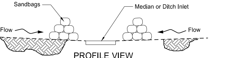
SANDBAG PROTECTION (LOW POINT)
