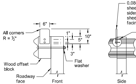
REFLECTORIZED PLATE DETAIL
