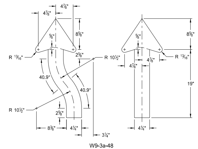
ARROW DETAILS
