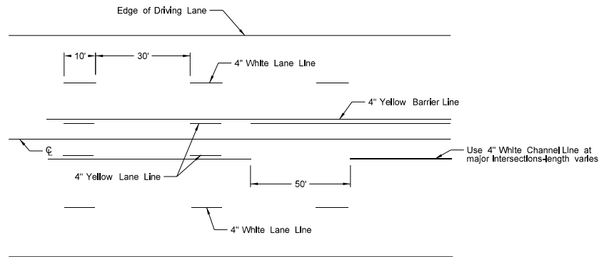
Painted or Tape Lines
