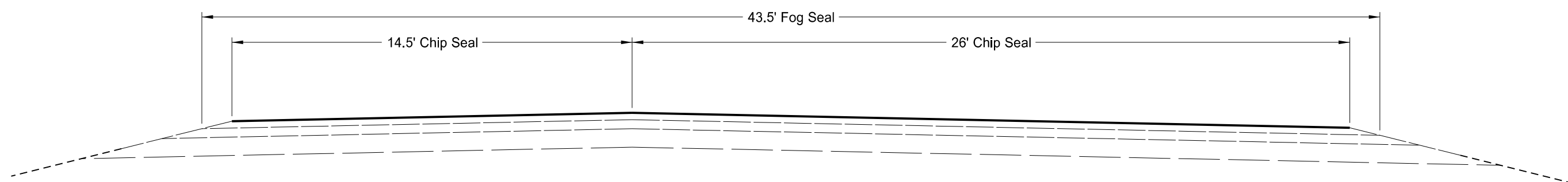
Proposed Typical Section (Climbing Lane) RP 45.155 to RP 45.466
