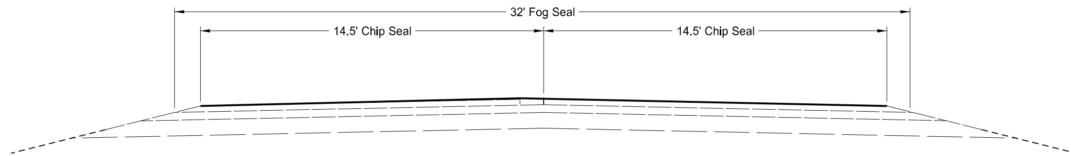
Proposed Typical Section RP 21.291 to RP 45.155 RP 45.466 to RP 45.762
