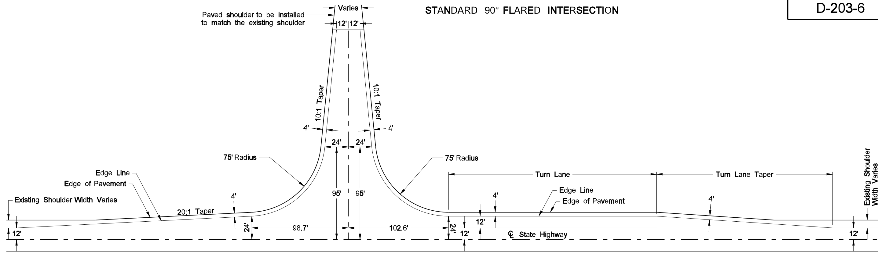
Type B 90° Flared Intersection with Turn Lane
