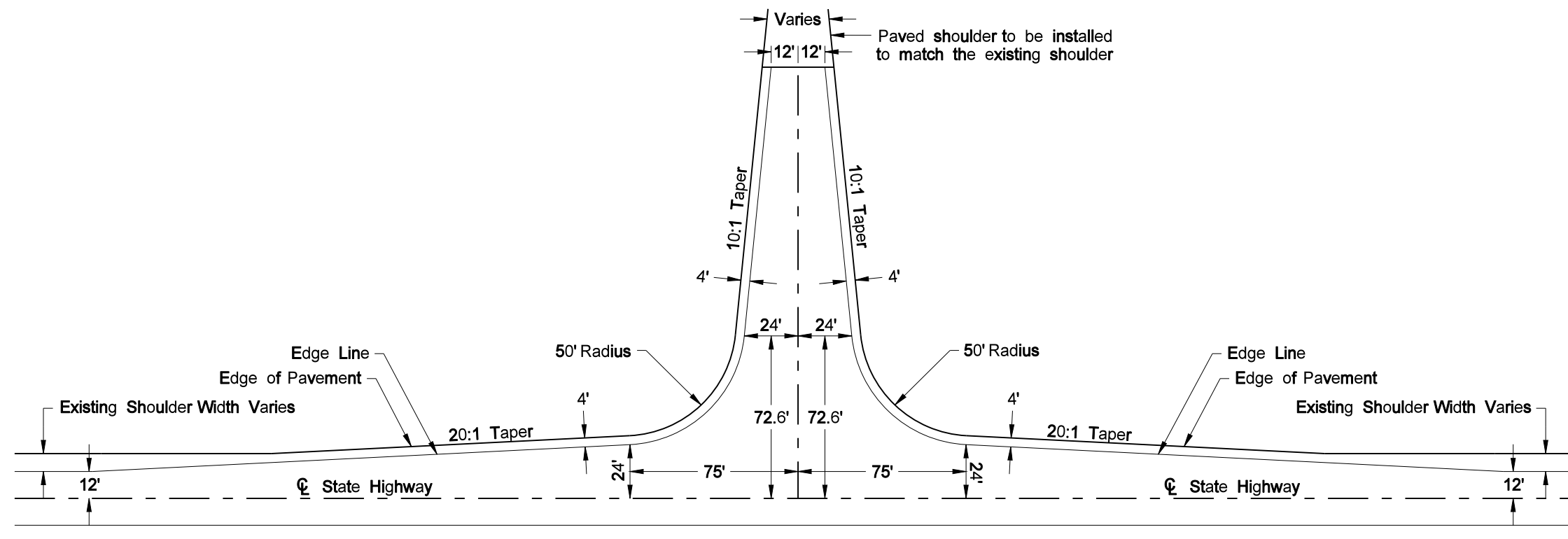
Type A 90° Flared Intersection
