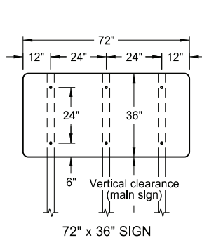
72" x 36" SIGN
