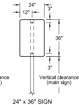
24" x 36" SIGN
