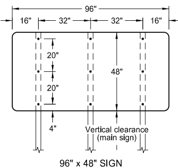
96" x 48" SIGN
