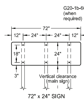
72" x 24" SIGN
