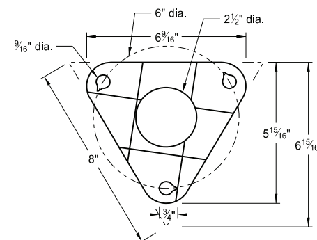
Bolt Retainer - 1/2" Reprocessed Teflon
