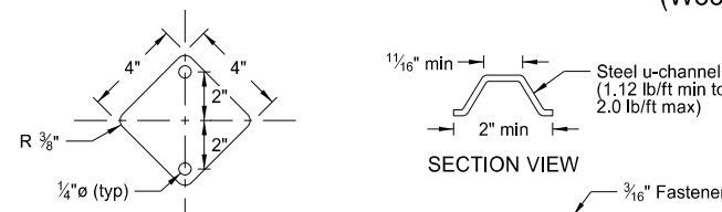
BARRICADE ASSEMBLY DETAIL (Wood or Plastic Rails)
