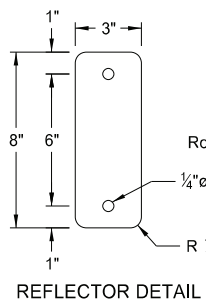
REFLECTOR DETAIL
