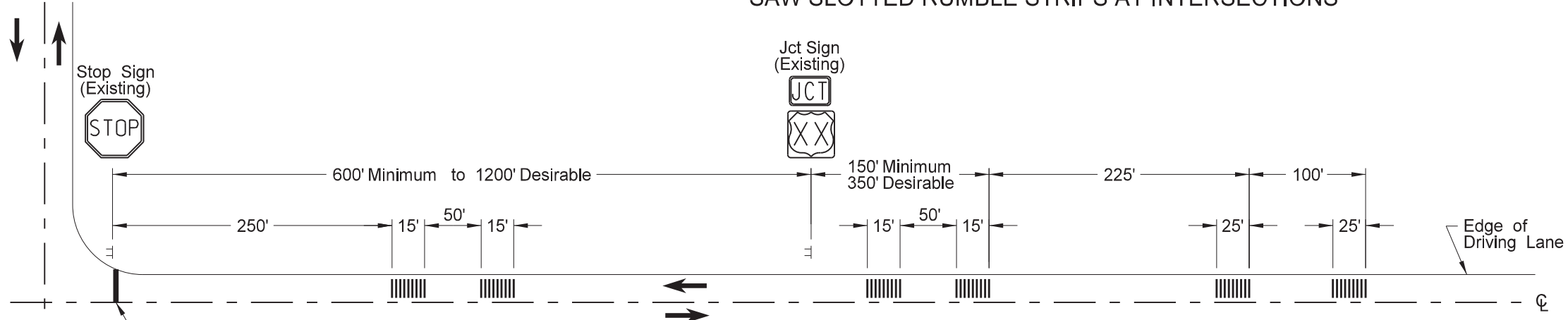
TYPICAL STOP INTERSECTION SAW SLOTTED RUMBLE STRIP LOCATION
