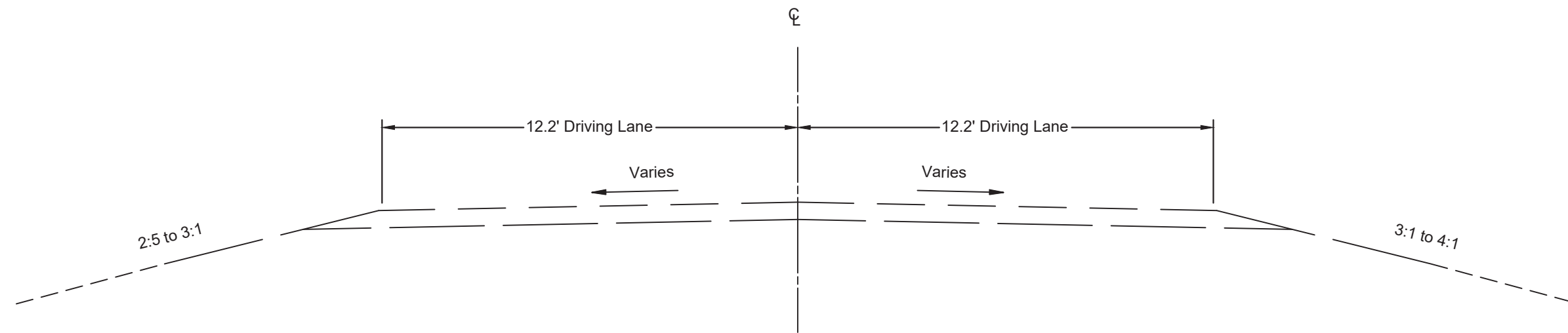
Existing Typical Section County Road 136 Sta. 10+00 to Sta. 59+70
