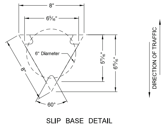
2 1/2" SQUARE POST RECEIVER Ductile Iron Casting class 65-45-12, Hot Dip Galvanize ASTM A153
