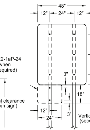
48" x 48" SIGN (with R2-1aP-24 sign as required)
