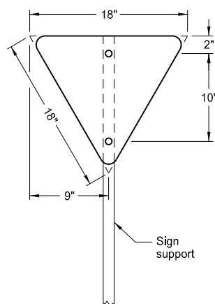
1 Post Assembly No. 101
