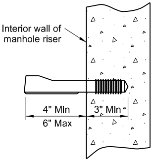
STEP DETAIL
